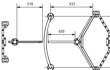
IDUN HBT3
