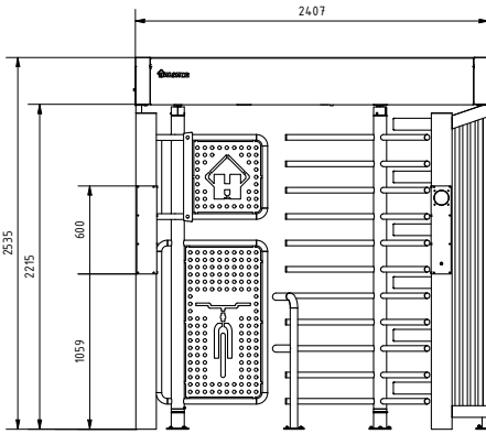
IDUN HBT3
